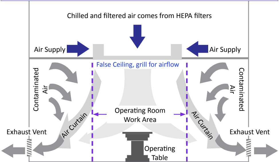
Working diagram of the air flow patterns in a Class 100 OT with Laminar Airflow and HEPA
